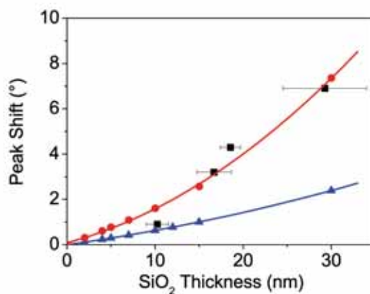
Figure 9.3: Measured peak shift of the reflection contrast as a function of the \text{SiO}_2 thickness (black squares), calculated peak shift of the reflection contrast for optimized polarization (red circles) and peak shift of a SPR sensor (blue triangles). The solid lines are fits to the data.
