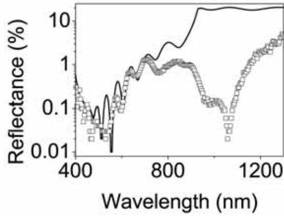
Figure 8.8: Measured (symbols) specular reflectance of sample XIX and fit using the transfer matrix method (curve) for an angle of incidence of 8^\circ .
