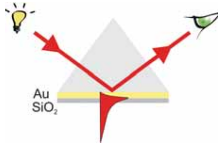
Figure 9.2: Surface plasmon polariton at the interface between gold and SiO 2 excited using total internal reflection on a prism-gold interface.
