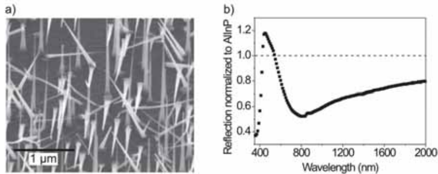
Figure 9.9: a) Scanning electron micrograph of GaP nanowires grown on AlInP that is lattice matched to GaAs. b) Total reflection from sample normalized to the total reflection of an AlInP layer grown on GaAs.
