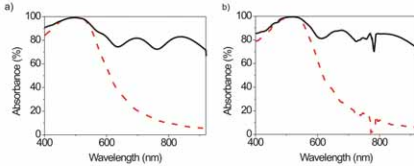
Figure 8.14: Simulated absorbance of base-tapered nanowires (black solid curve) and straight nanowires (red dashed curve) for a) normal incidence and b) an angle of incidence of 30°.
