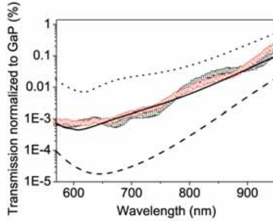
Figure 6.13: Measured transmitted intensity through a nanowire layer with a thickness of 1.6\ \mu\text{m} grown on a (100) GaP substrate (sample XVI on page 29) for azimuthal angles of 0^\circ (black squares) and 90^\circ (red circles) normalized to the transmitted intensity through a bare GaP substrate. The calculations of the transmission for a nanowire diameter distribution varying between 115 nm to 155 nm and the angle of incidence varying between 10^\circ and 50^\circ are included for s-polarized (dotted curve) and p-polarized (dashed curve) light. The average of the two calculations is displayed with the solid curve.
