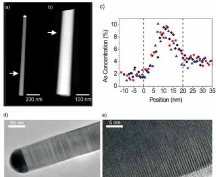
Figure 8.15: Transmission electron micrographs of a nanowire removed from sample XIX a) low resolution and b) zoom-in to the heterostructure. c) EDX linescans from three wires of the same sample along the heterostructure. d) low resolution and e) high resolution TEM images of the top part of the wire. In d) the gold particle that catalyzes the growth of the nanowire is visible. The high resolution TEM image in e) reveals the wurtzite crystal structure of the nanowires.
