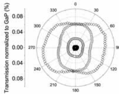
Figure 6.14: Measured transmission through a nanowire layer with a thickness of 1.6\ \mu\text{m} grown on a (100) GaP substrate (sample XVI on page 29) normalized to the transmission through a bare GaP substrate as a function of azimuthal angle for a wavelength of 750 nm (filled squares), 800 nm (open circles), 850 nm (open triangles), 900 nm (open diamonds).
