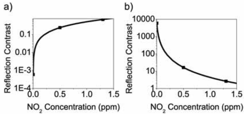
Figure 9.6: Calculated reflection contrast as a function of \text{NO}_2 concentration for of a layer of GaP nanowires with a length of 1.5 \mu\text{m} , a GaP filling fraction of 15 %, and an angle of incidence of 60^\circ at a wavelength of a) 700 nm and b) 730 nm. The symbols correspond to the calculated reflection contrast of Fig. 9.5, the curves are parabolic fits.
